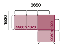
Бл-1у(900)-1у(900)-У-1у(900)-Бп
