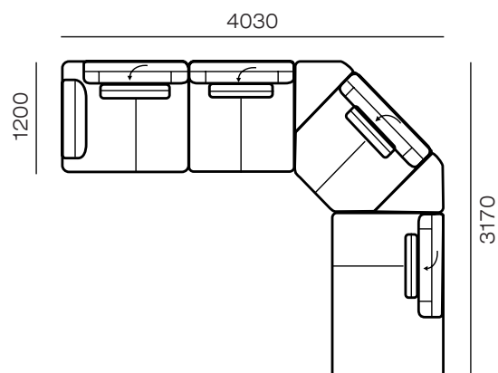
Бл-1у(1100)-1у(1100)-У-1у(1100)
