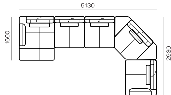
Бл-К(1100)-1у(1100)-1у(1100)-У-1у(1100)-Бп
