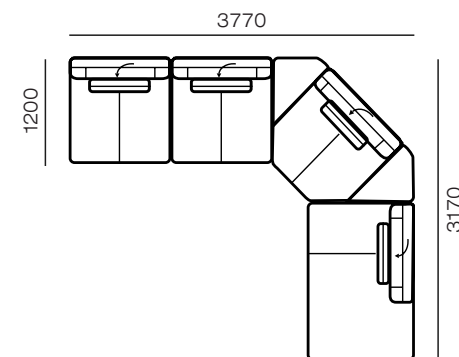
1у(1100)-1у(1100)-У-1уб(1100)
