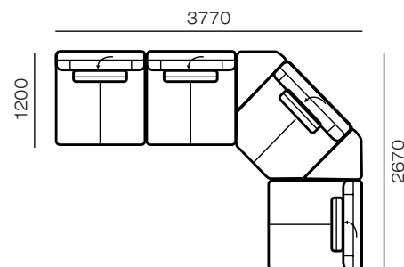
1у(1100)-1у(1100)-У-1у(1100)
